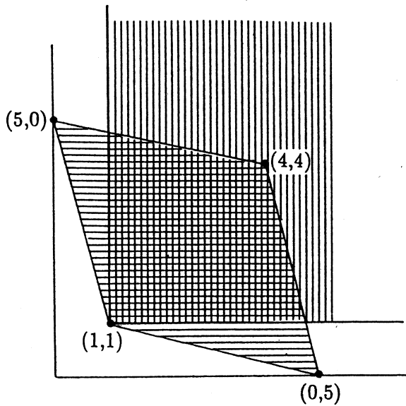
Figure 1 Feasible and individually rational payoffs in the Prisoner's Dilemma.
